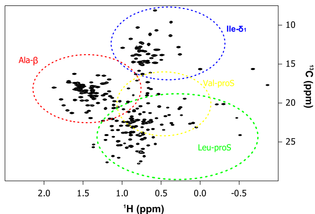
Fig. 7 2D [ ^1\text{H} , ^{13}\text{C} ] spectra of [ U - ^2\text{H} ], A- [\text{}^{13}\text{CH}_3]^\beta , I- [\text{}^{13}\text{CH}_3]^\delta , (LV)- [\text{}^{13}\text{CH}_3]^{\text{proS}} MSG (82 kDa). MSG sample was produced with scrambling-free and incorporation optimized combinatorial labeling protocol described in “Materials and methods” section. Spectra were acquired at 37 °C on a spectrometer operating at a proton frequency of 800 MHz. The sample concentrations was 1 mM in ^2\text{H}_2\text{O} buffer at pH 7.1 containing 20 mM MES and 25 mM \text{MgCl}_2 . In blue circle \text{I}^\delta signals, in red circle \text{A}^\beta signals, in yellow circle \text{V}^{\text{proS}} signals and green circle \text{L}^{\text{proS}} signals
