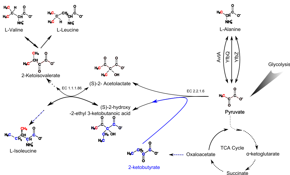
Fig. 2 Biosynthetic pathway of the AILV residues. The pathway for the scrambling of ^{13}\text{C}_3 group from alanine into isoleucine, leucine and valine is indicated in red . The carbons from 2-ketobutyrate are depicted in blue . Each biosynthetic intermediate has been named according to the Kyoto Encyclopedia of Genes and Genomes (KEGG). The enzymes responsible for catalyzing each reaction are
