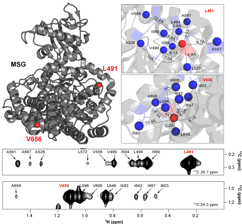
Fig. 8 Detection of long-range nOes in the [ U -D], A- [\text{}^{13}\text{CH}_3]^\beta , I- [\text{}^{13}\text{CH}_3]^\delta , (LV)- [\text{}^{13}\text{CH}_3]^{\text{proS}} -MSG sample (82 kDa). 2D extracts of the 3D ^{13}\text{C} -HMQC-NOESY spectrum are presented along with the extracted distances between each pair of methyl groups from the 3D structure of MSG (1D8C; Howard et al. 2000). The experiment was acquired on a 800 MHz spectrometer equipped with a cryoprobe at 37 °C for 3.5 days with recycling delay d_1 = 1.3 s and NOE mixing time \tau_m = 500 ms. The [ U - ^2\text{H} , \text{A}^\beta\text{I}^\delta(\text{LV})^{\text{proS}} ]-MSG sample was at 1 mM in a ^2\text{H}_2\text{O} buffer containing 20 mM MES, pH 7.1, and 25 mM \text{MgCl}_2 . Diagonal peaks are labeled by residue numbers in red and nOes cross-peaks in black
